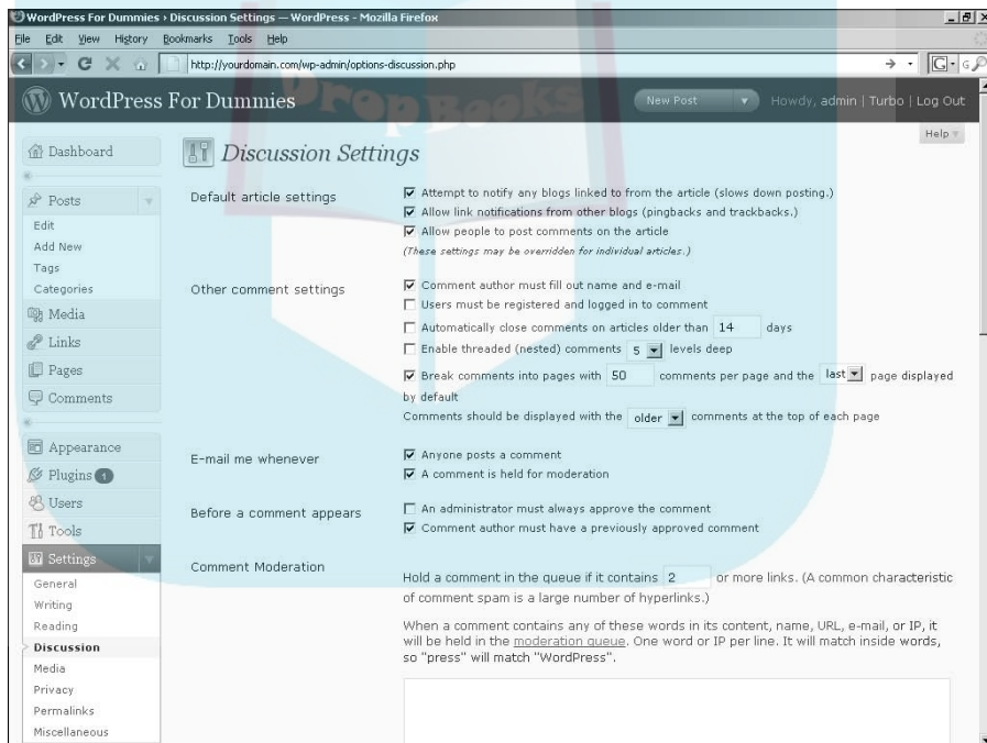
Figure 7-13: The Discussion Settings page.
